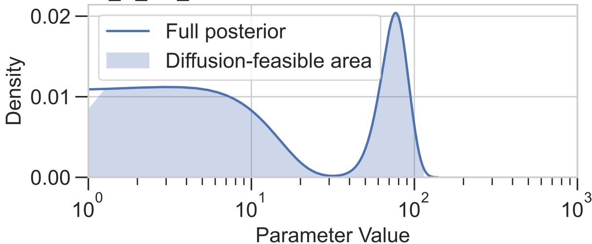
kon_D_Act_ACP: Posterior with Diffusion-Feasible Area
